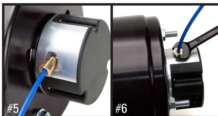
INSERT FITTING AND AIRLINE INTO AIR SPRING
